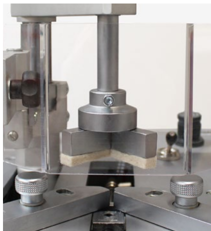
Magnetic pad holder and L-shaped pad with felt
